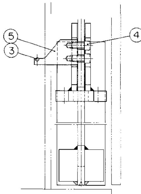
SECTION "A-A"
