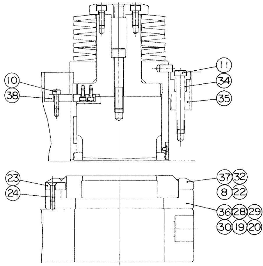
4-1/2"-56st
