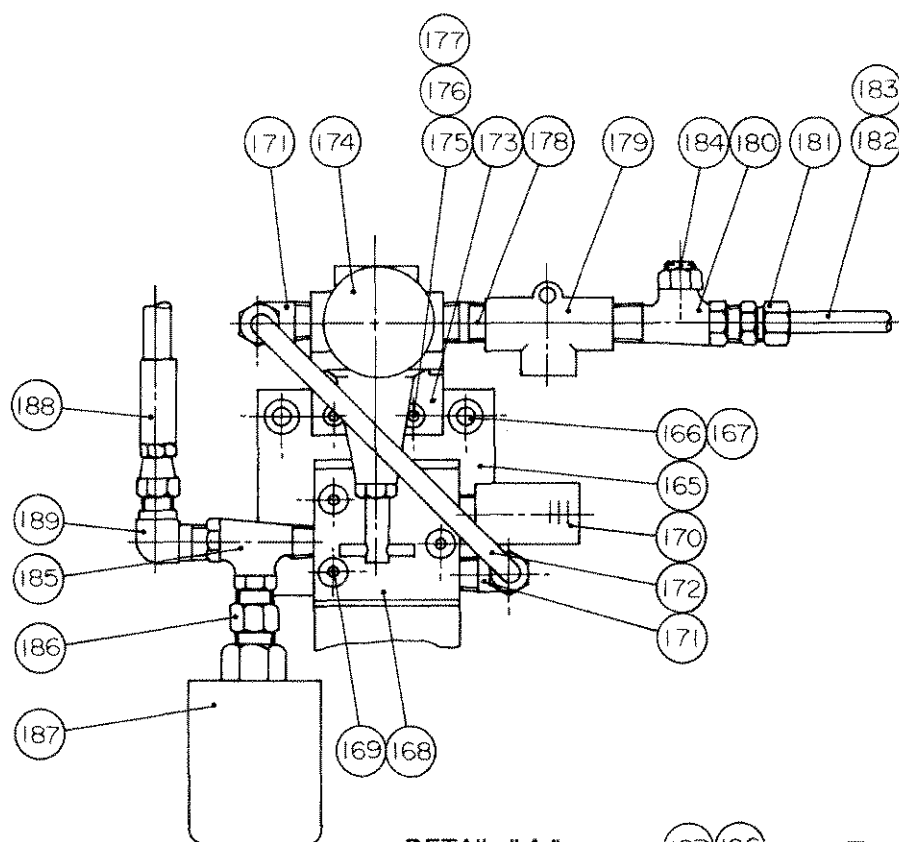
DETAIL "A"
